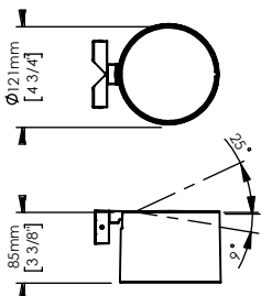
CM CORNER WALL-MOUNTING
